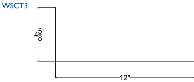
"Chimney/Skylight Top Flashing"
