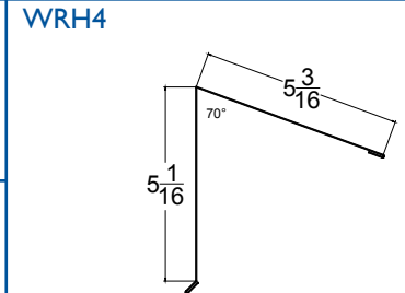
"Monoslope Ridge Flashing"
