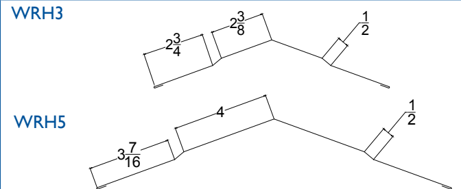
"Standard Ridge Flashings"
