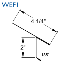
"Eave Flashings"
