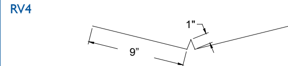
"Valley Flashing"
