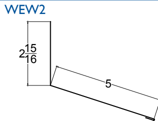
"J-Channel Flashing"
