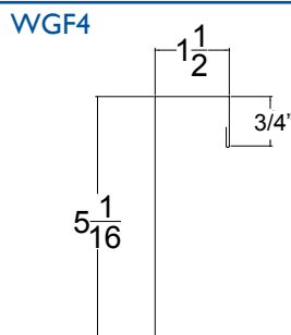
"Gable Flashing"
