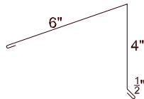
MONOSLOPE PEAK CAP CP-1
