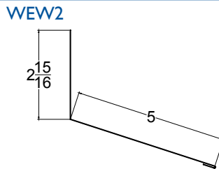
"J-Channel Flashing"
