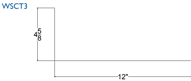
"Chimney/Skylight Top Flashing"
