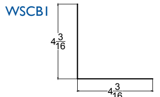
"Chimney/Skylight Bottom Flashing"
