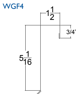
"Gable Flashing"
